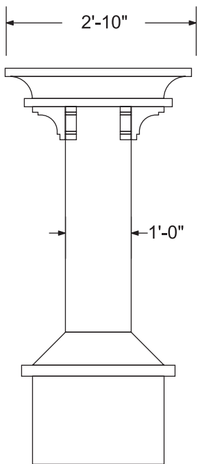
End View
